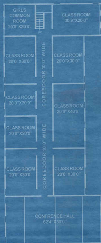
BASEMENT FLOOR PLAN BLOCK-A
