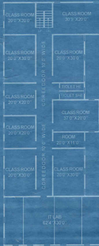
FIRST FLOOR PLAN BLOCK-A
